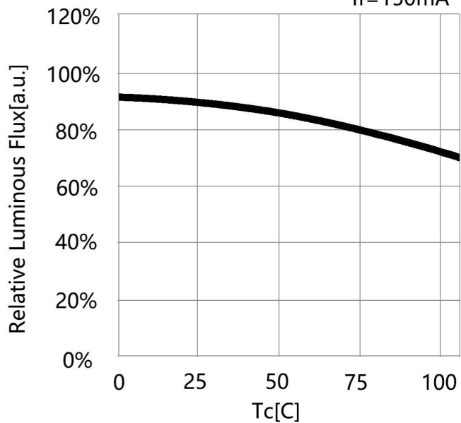
Case Temperature vs. Relative Luminous Flux I F =150mA
