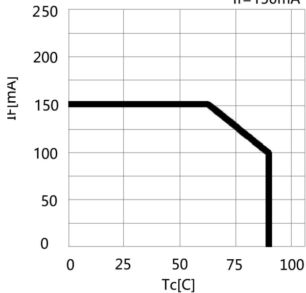
Case Temperature vs. Forward Current I F =150mA
