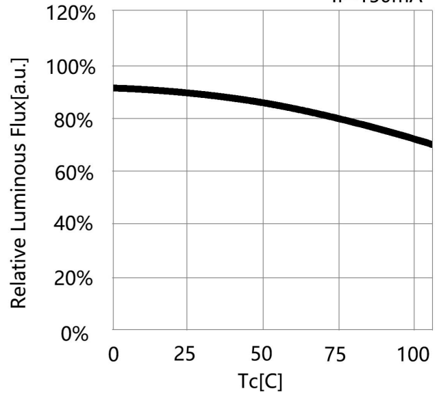
Case Temperature vs. Relative Luminous Flux If=150mA
