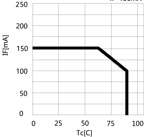
Case Temperature vs. Forward Current If=150mA
