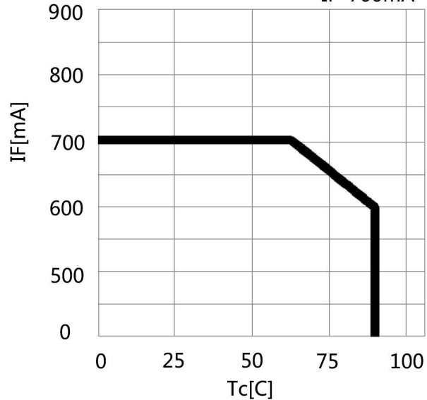
Case Temperature vs. Forward Current If=700mA
