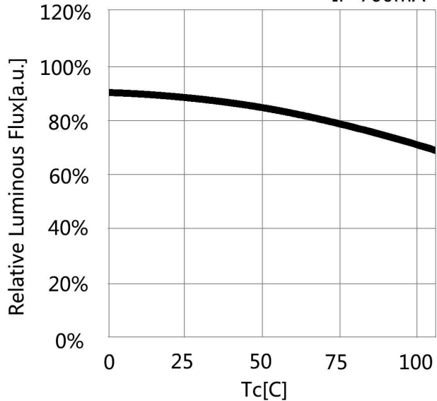
Case Temperature vs. Relative Luminous Flux If=700mA
