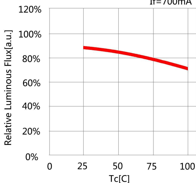
Temperature vs. Relative Luminous Flux I F =700mA
