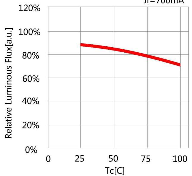
Temperature vs. Relative Luminous Flux I F =700mA
