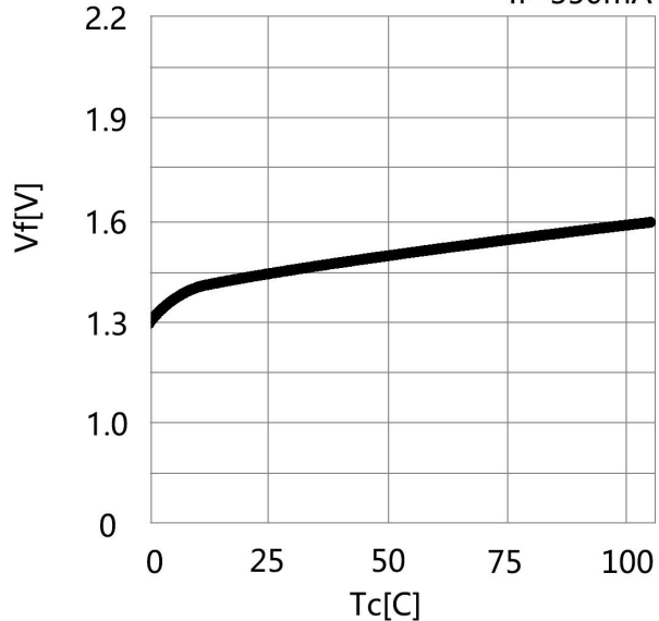
Case Temperature vs. Forward Voltage I f =350mA
