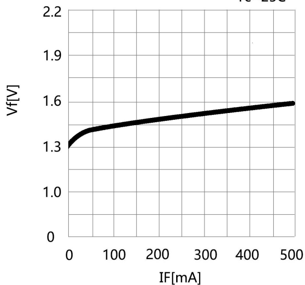
Forward Current vs. Forward Voltage T c =25C
