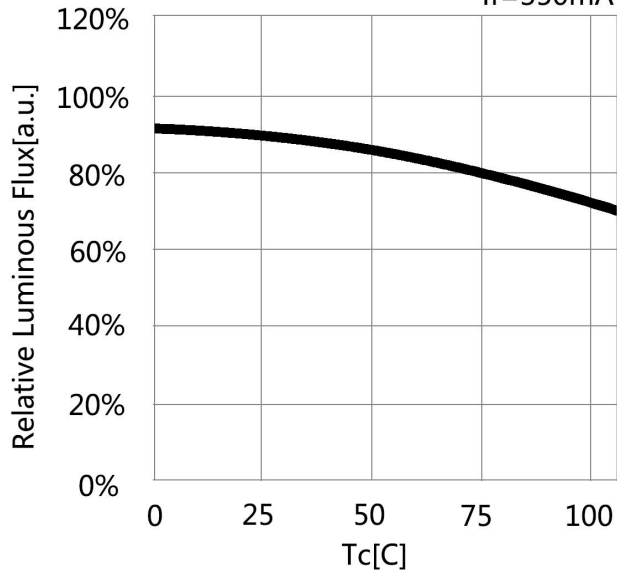
Case Temperature vs. Relative Luminous Flux I f =350mA
