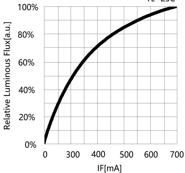
Forward Current vs. Relative Luminous Flux T c =25°C
