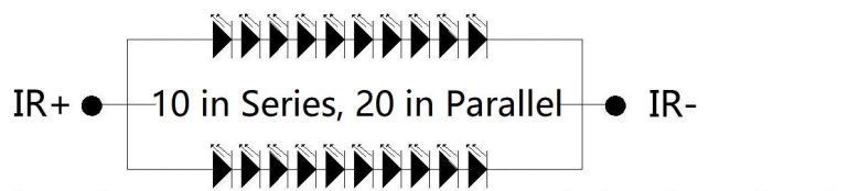
(Cathode-) Circuit diagram
