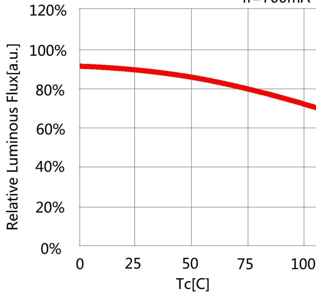
Case Temperature vs. Relative Luminous Flux I f =700mA
