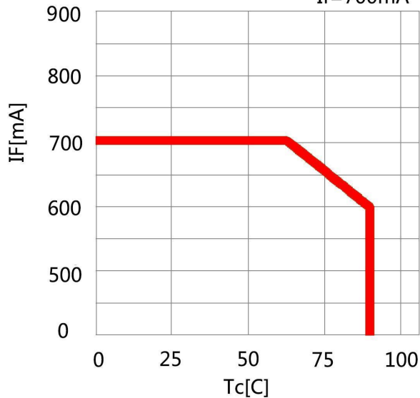
Case Temperature vs. Forward Current If=700mA
