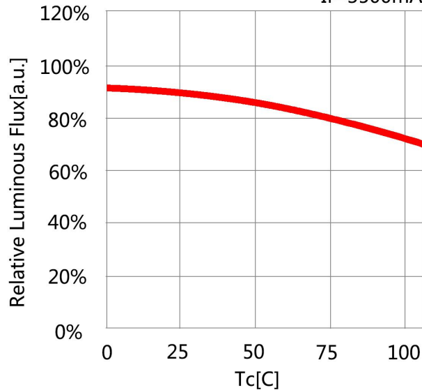
Case Temperature vs. Relative Luminous Flux I f =3500mA
