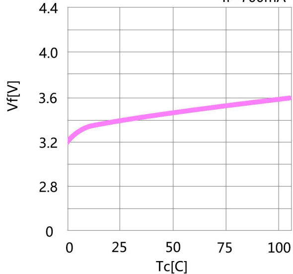
Case Temperature vs. Forward Voltage I f =700mA
